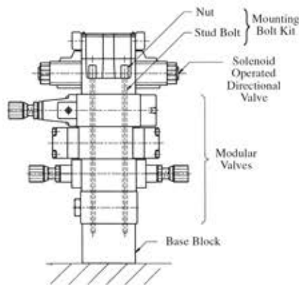
03 Series Modular Valve Assembly
